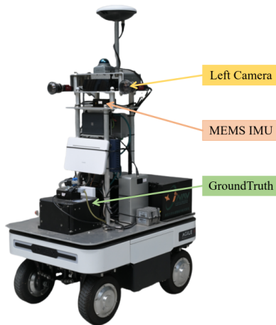
Fig. 8. Wheeled robot platform for the i2Nav-Robot dataset.
