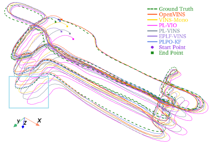
Fig. 13. Resulting trajectories of the HandNav hybrid01 sequence. All trajectories start from the same point and end at different starts, each shown in a distinct color.
